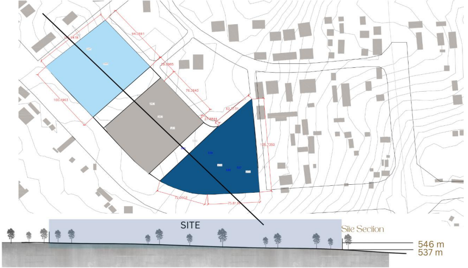
SITE SECTION
