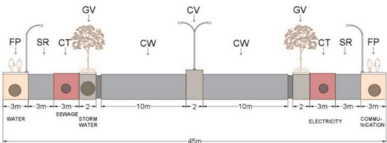
ROAD SECTION
